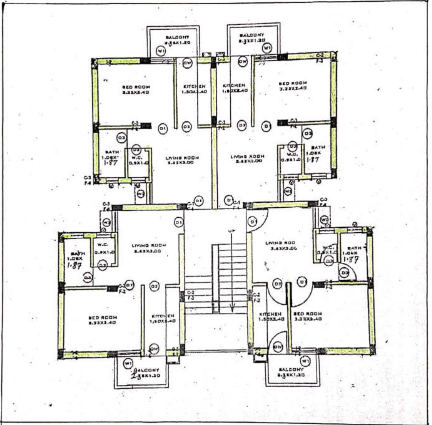
EWS(G+2) Flats Building Plan (1-BHK) Plinth area = 33.707 Sqm.
