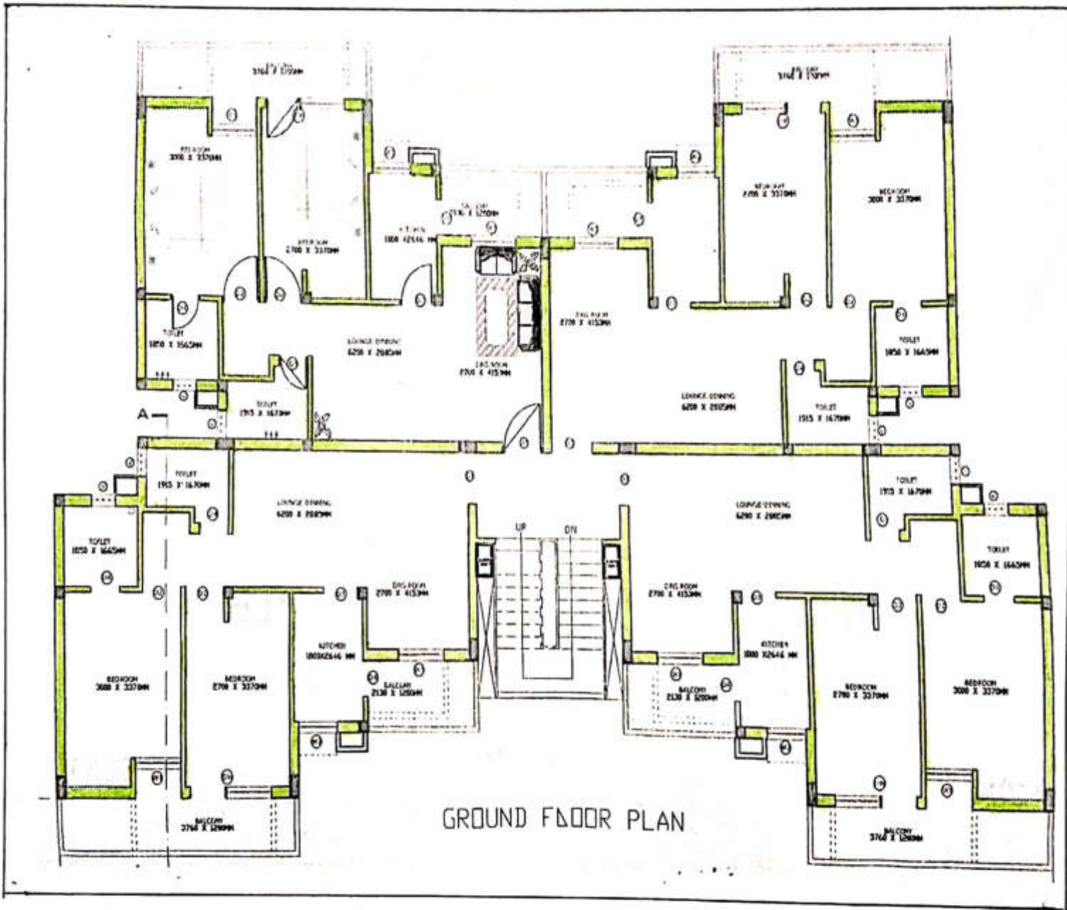
MIG-A(G+2) Flats Building Plan (2-BHK) Plinth area = 76.037 Sqm.
